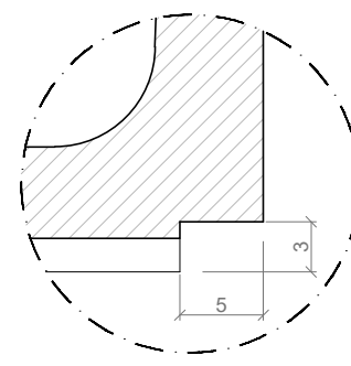
DETALLE B / DETAIL B
